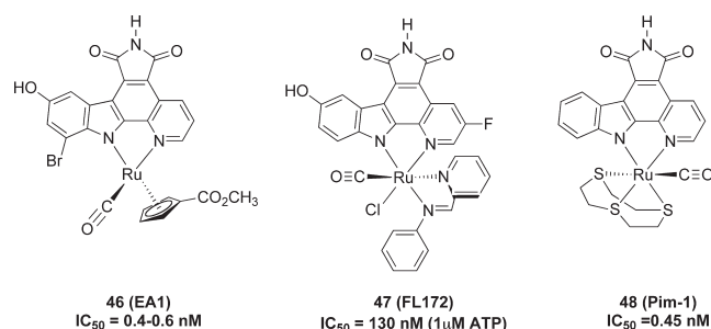
Figure 18. Examples of Ru(II) organometallics as kinase inhibitors with their IC_{50} values. IC_{50} values were measured at 100 \mu M ATP if not indicated otherwise.
