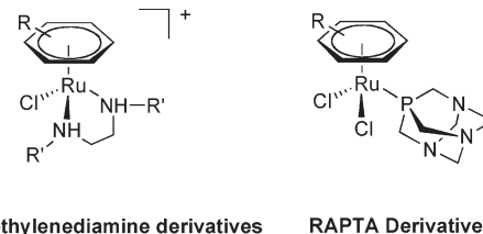
Figure 7. (\eta^6\text{-Arene}) ruthenium anticancer complexes.
