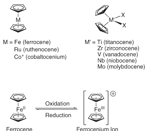
Scheme 1. (Top Row) Classical Metallocenes with Parallel Cp Rings (Left) and Bent Metallocenes (Right) with the Medically Relevant Metals Indicated and (Bottom Row) Reversible Oxidation Chemistry of Ferrocene
